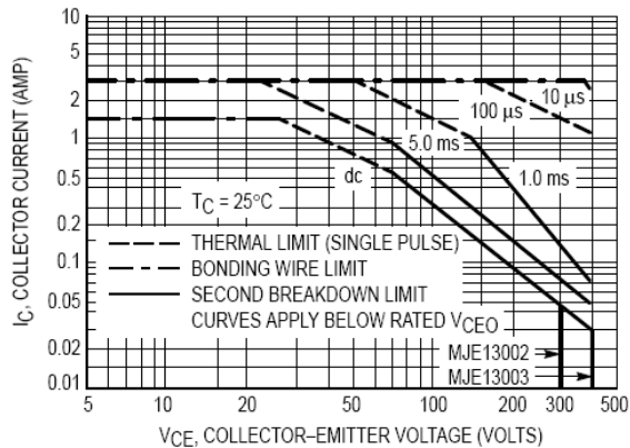
Figure 11. Active Region Safe Operating Area
