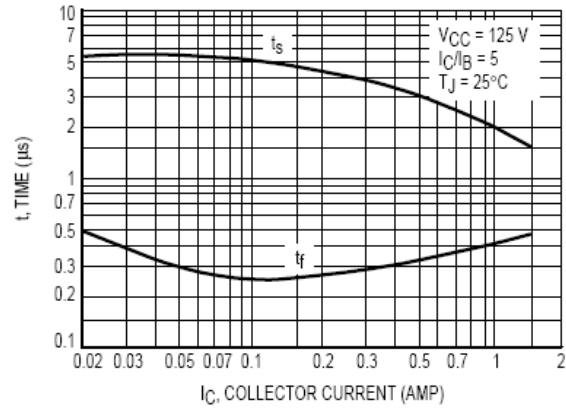
Figure 9. Turn-Off Time
