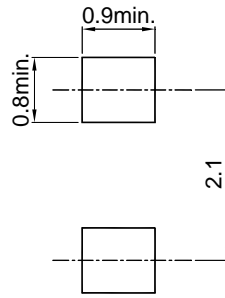
SOD-323
