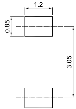
SOD-123
