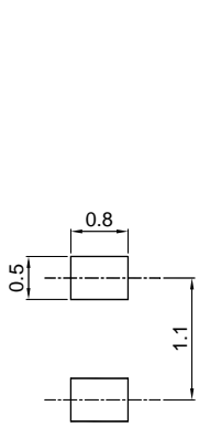
SOD-723
