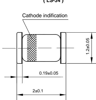
Glass case QuadroMELF Dimensions in mm (LS-34)
