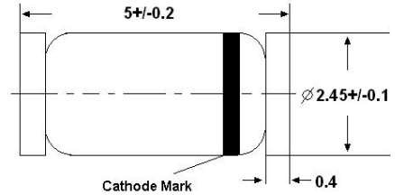
Glass case MELF Dimensions in mm (LL-41)
